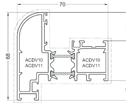
DV21 Rounded Sash Profile Available On Open In & Open Out Doors
