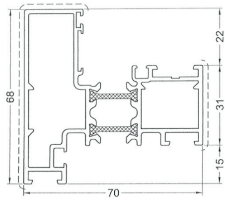
DV121 Square Sash Profile Only Available On Open Out Doors
